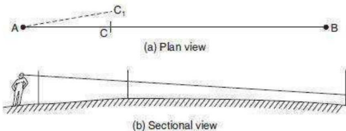
Figure 7: Direct Ranging
