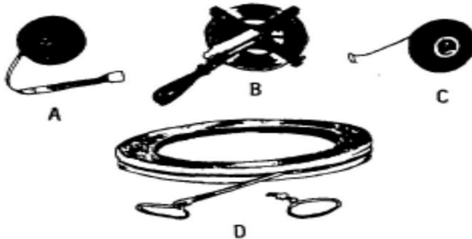
Figure 2: Surveying tapes.
