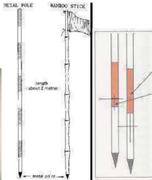
Figure 4: Ranging rods
