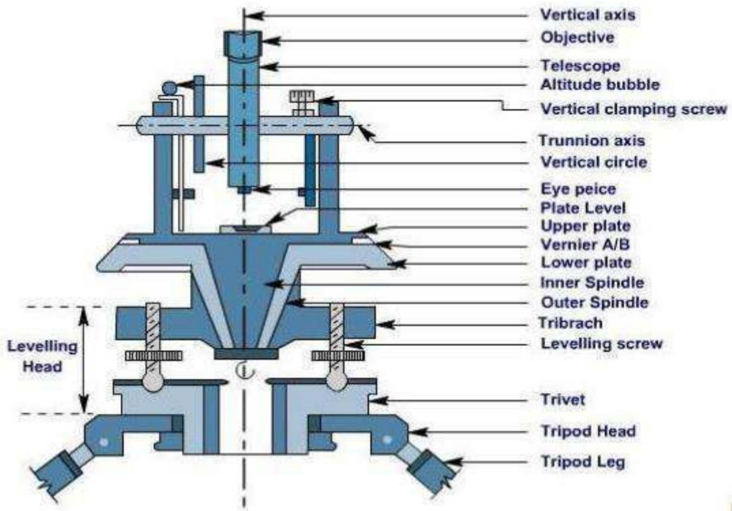
Sectional view of theodolite
