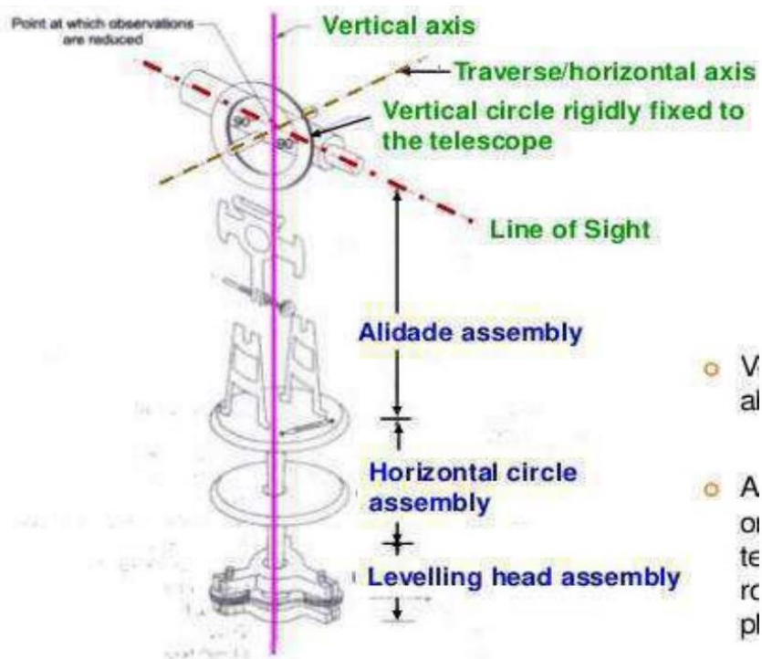
Three assemblies of theodolite
