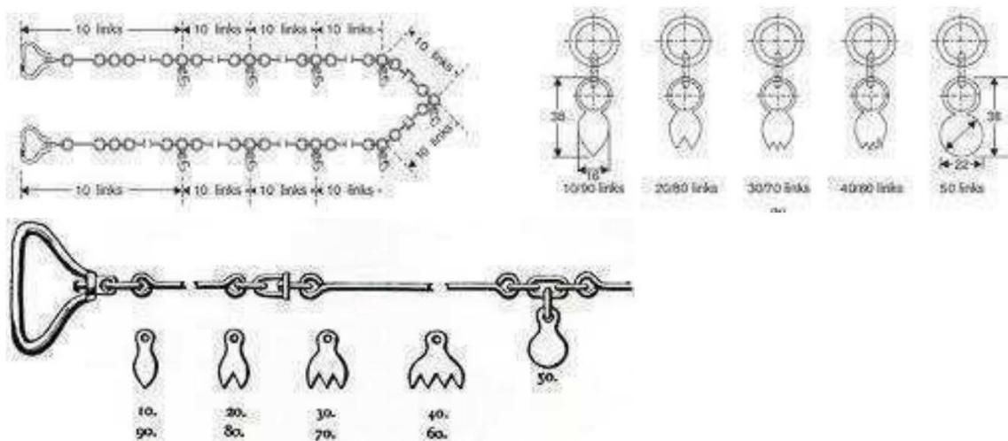
Figure 1: Chains
