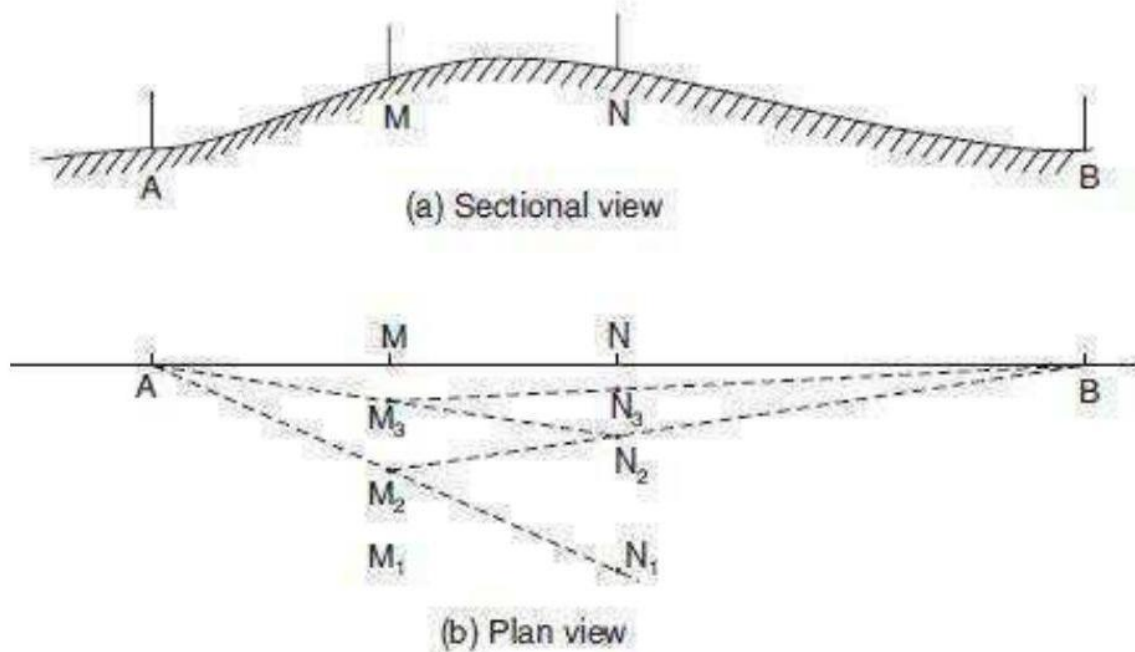
Figure 8: Indirect or Reciprocal Ranging
