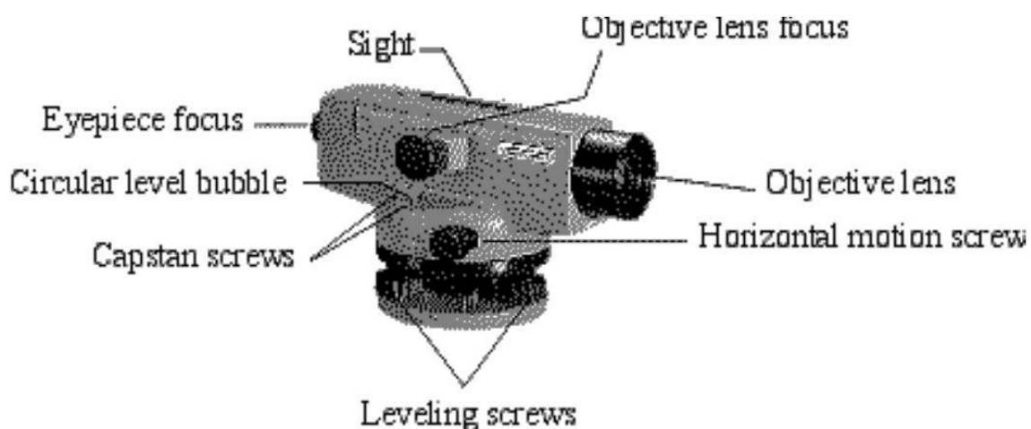
Figure 15: Parts of Level
