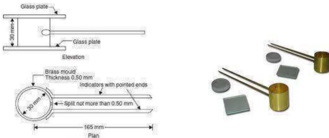
Figure 4: Le Chatelier apparatus
