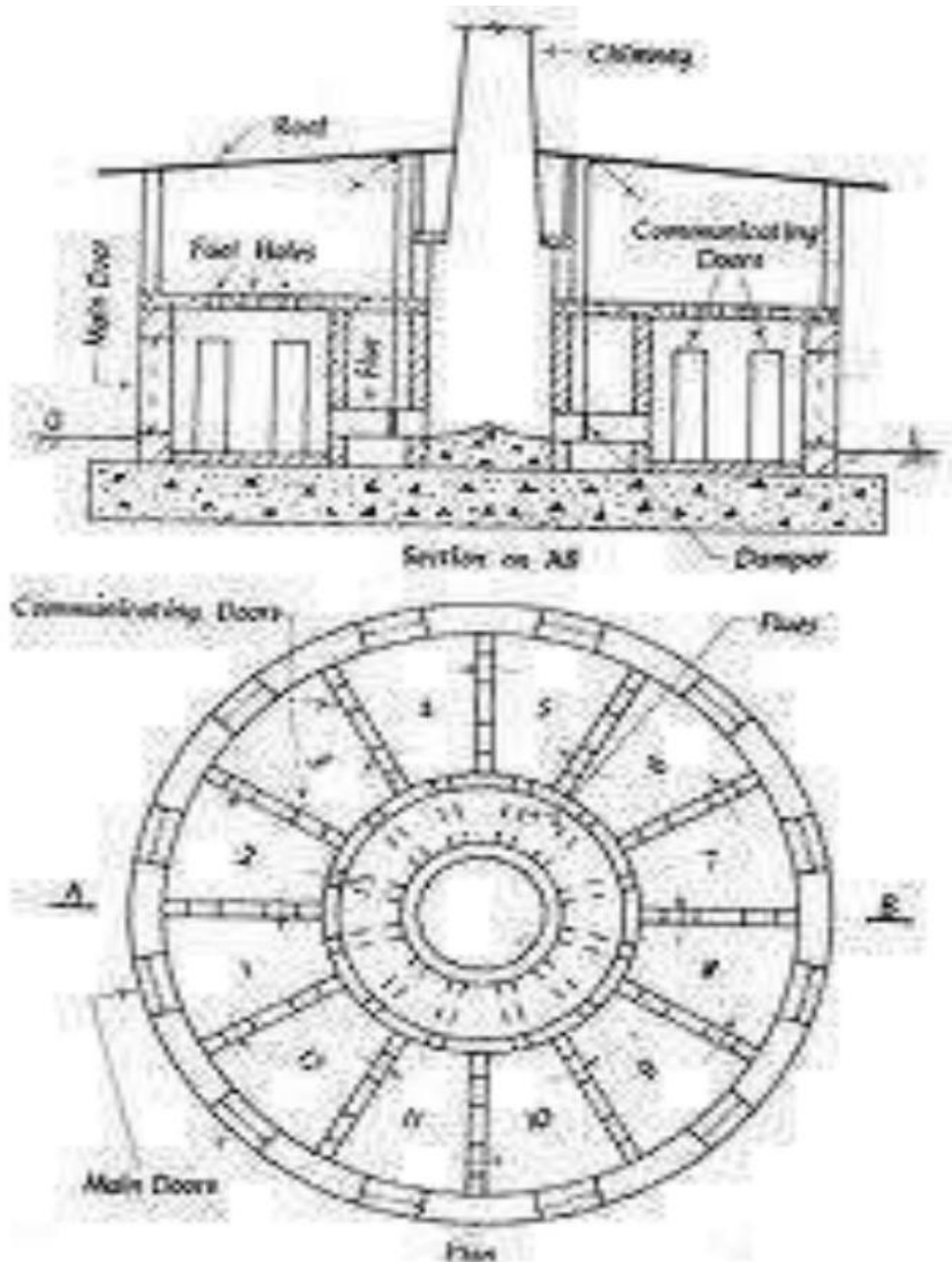
Figure 2: Bull's Trench Kiln
